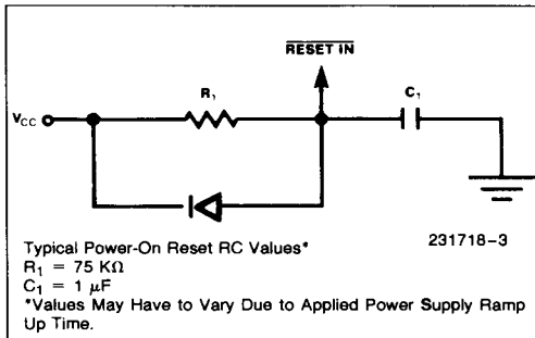
Figure 3. Power-On Reset Circuit
